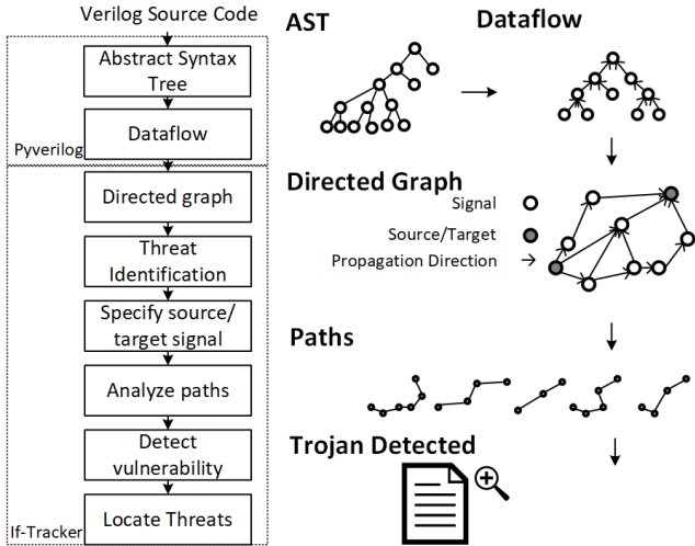
Fig. 1: Workflow of the proposed If-Tracker framework.
